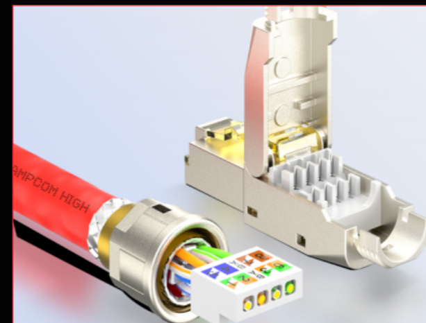
Tool Free Crimping Even Novices Can Easily Connect Wires
