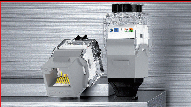
Lock-Free No Crimping Cat6A Unshielded Network Module - Grey
