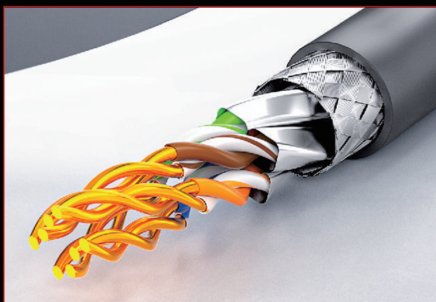
99.95% Oxygen-Free Copper with Aluminum Braid Shielding.
