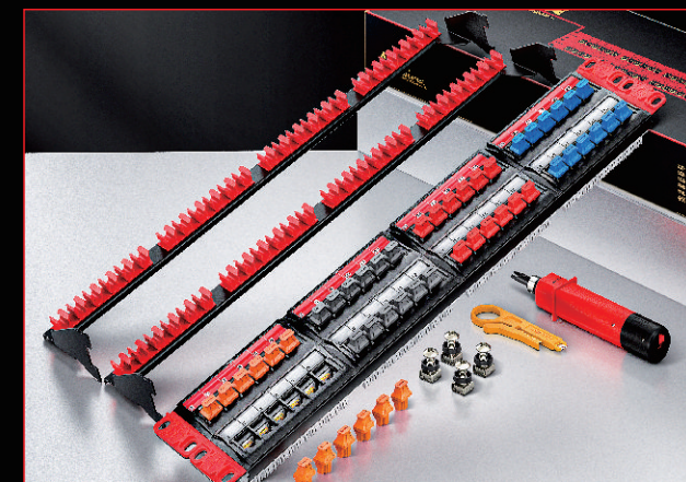
2U 48-Port Cat6 Unshielded 19-Inch Patch Panel
